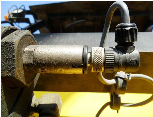
Typical Pressure Transducer Installation
